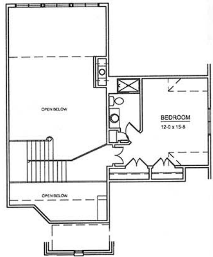
Optional Second Floor Plan (adds dormer to elevation)
